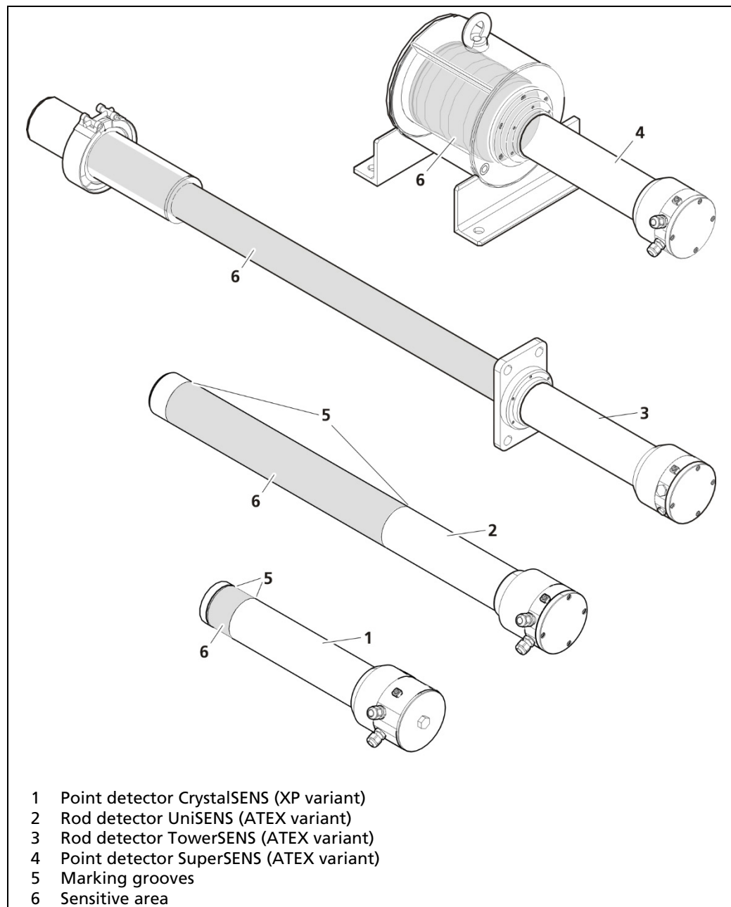
Fig. 4 View of the DuoSeries detectors
