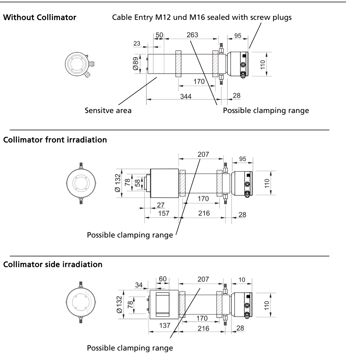
TI-Fig. 2 Dimensions CrystalSENS LB-4700-1x with water cooling (Dimensions in mm)
