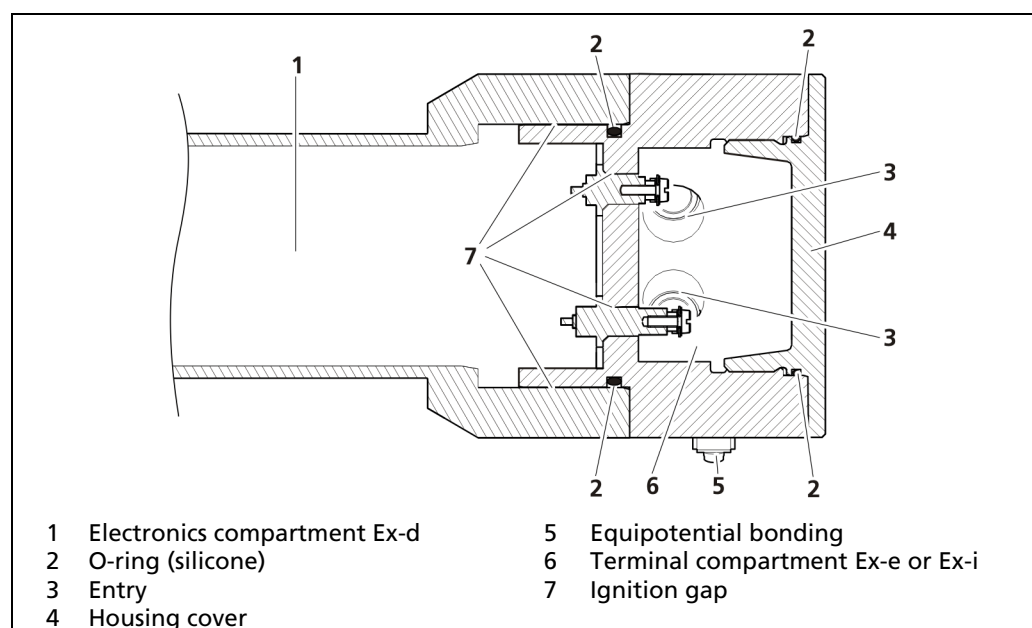
Fig. 3 Explosion Protection Design LB 4700-xx-Fx
