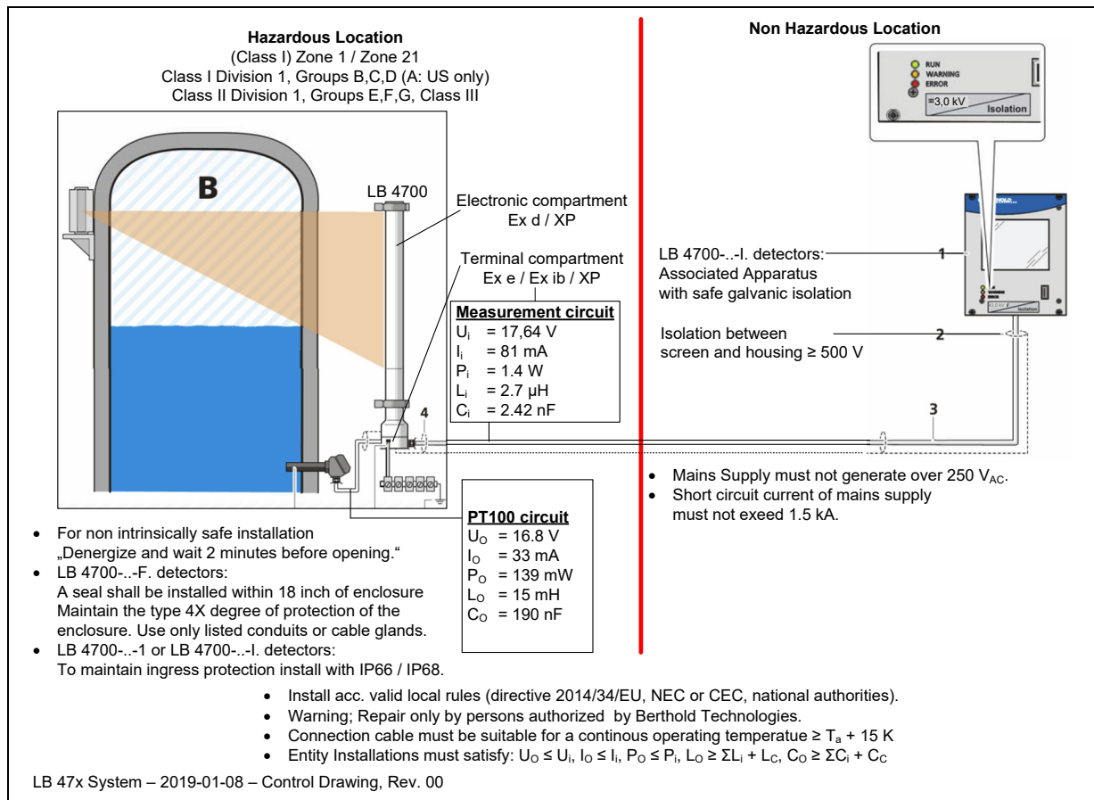
Fig. 1 Control Drawing
