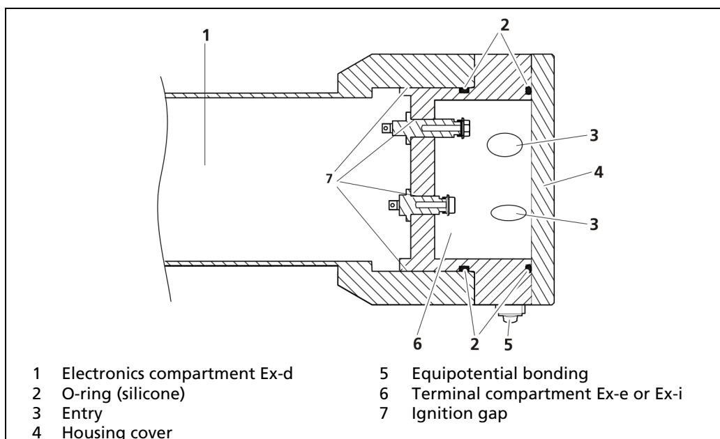
Fig. 2 Explosion Protection Design LB 4700-xx-1x / LB 4700-xx-lx
